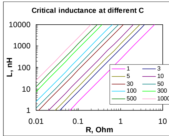
Figure 11. Critical inductance vs. total resistance of the circuit. The legend shows values of capacitors in \mu F .
